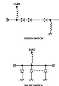
Figure 4 - Reflective Spst Switch
