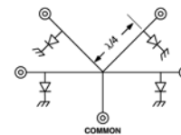
Figure 2b - Shunt Diodes Located Quarter Wave Length from Common Junction
